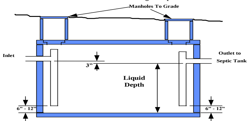
Figure 7 - Grease Interceptor Tank
