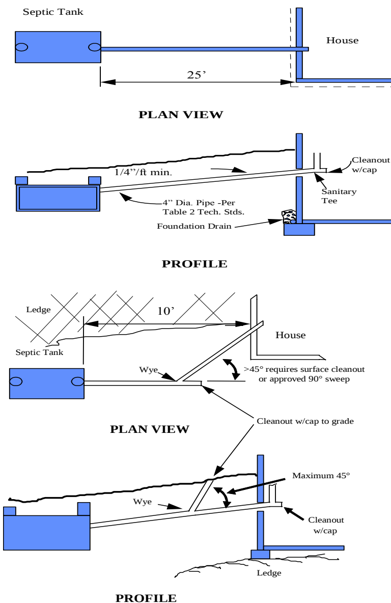
Figure 1 - Building Sewers
