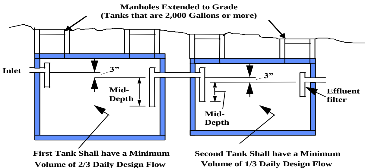
Figure 5 – Septic Tanks in Series
