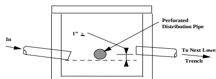
Reversed Distribution Box
