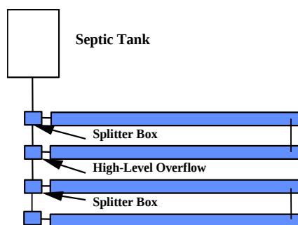
Figure 10 - Alternative Distribution Systems & D-Boxes
