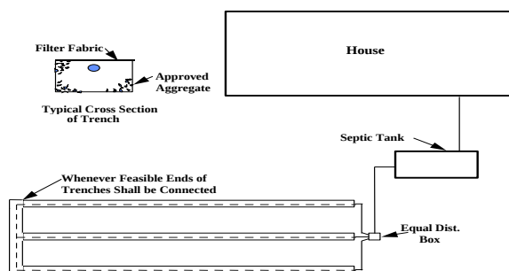
Figure 8 - Level Leaching Systems
