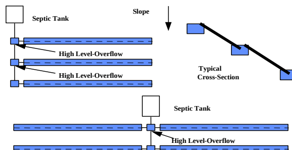
Figure 9 - Serial Distribution Systems
