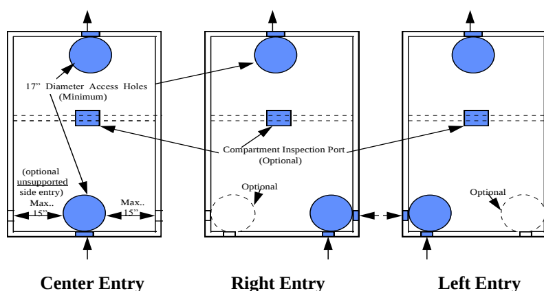
Figure 6 – Standard Septic Tank Configurations
