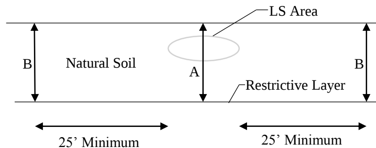
Diagram 2 - Flat Groundwater Table
