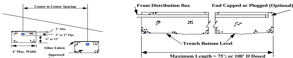
Figure 14 - Leaching Trenches
