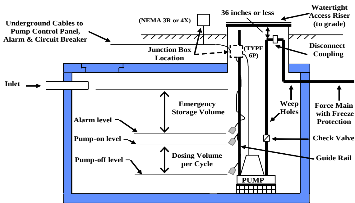
Figure 11 - Pump Chamber
